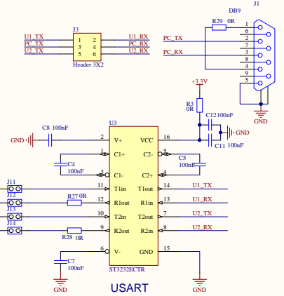
USART
