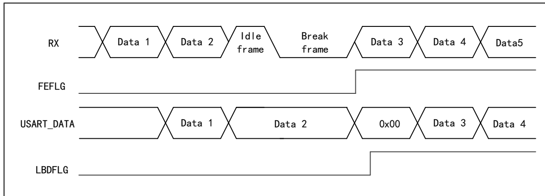
Figure 99 Break Frame Detection in Idle State
