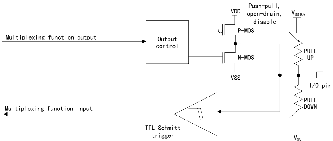
Figure 22 I/O Structure in Multiplexing Mode
