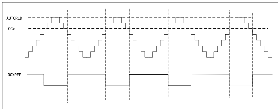
Figure 74 PWM1 Center Alignment Mode Timing Diagram
