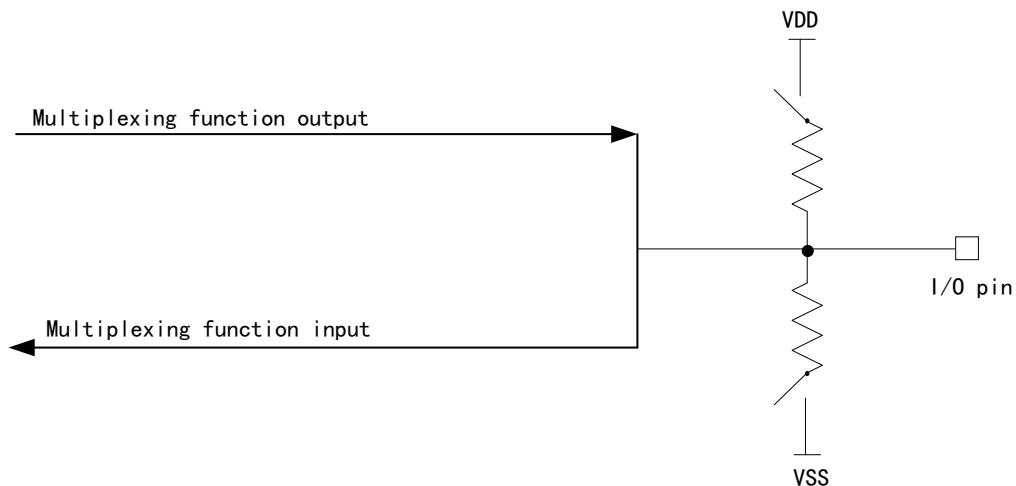
Figure 21 Analog Function I/O Structure
