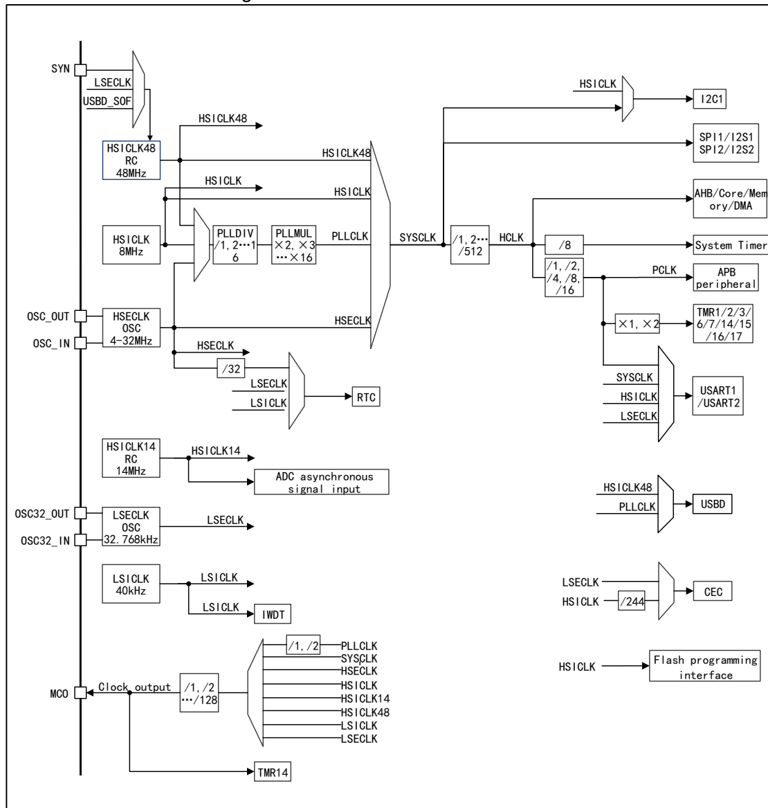
Figure 4 APM32F072x8xB Clock Tree
