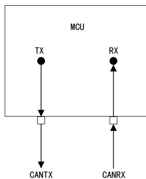
Figure 131 CAN Works in Normal Mode
