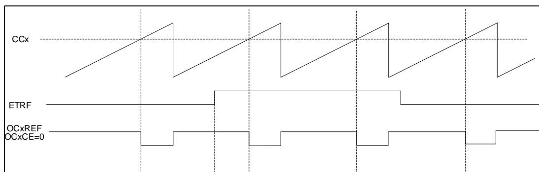
Figure 86 OCxREF Timing Diagram
