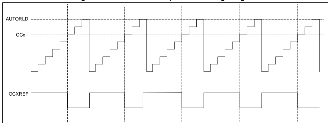
Figure 56 PWM1 Count-down Mode Timing Diagram
