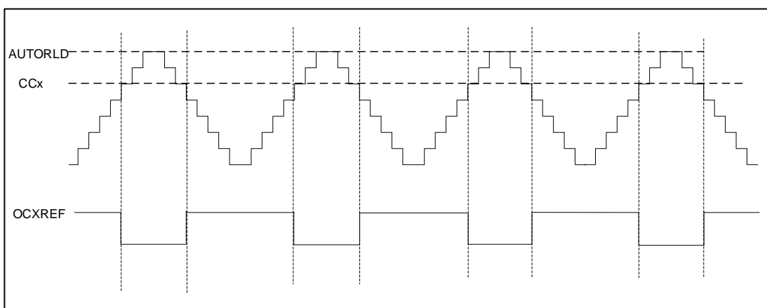
Figure 47 PWM1 Center-aligned Mode Timing Diagram
