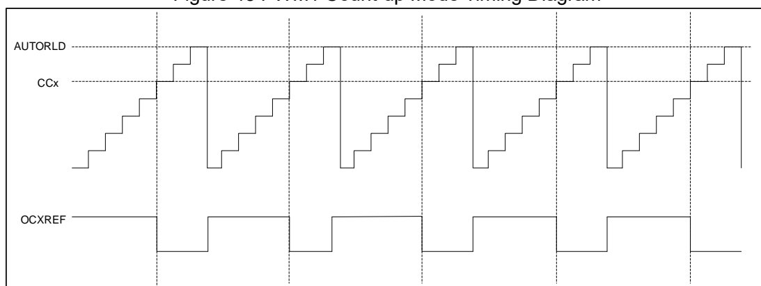
Figure 46 PWM1 Count-down Mode Timing Diagram
