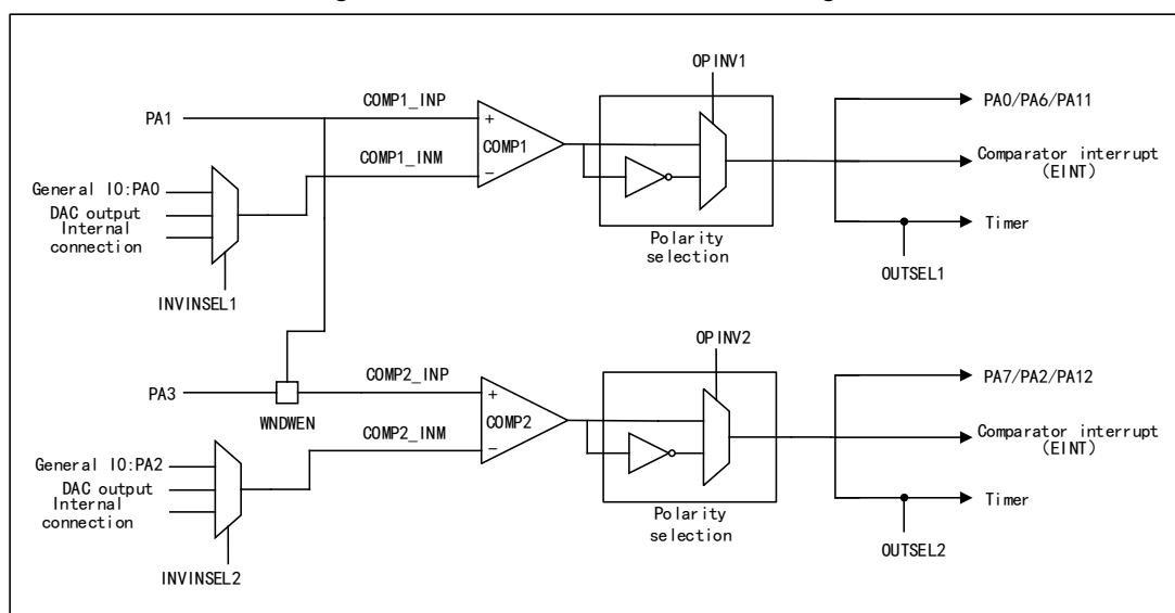
Figure 128 COMP Structure Block Diagram
