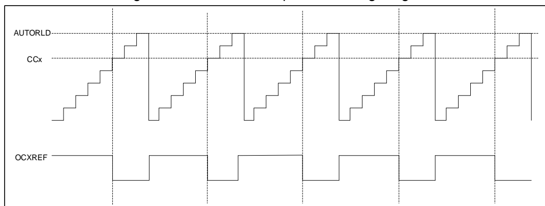
Figure 29 PWM1 Count-up Mode Timing Diagram
