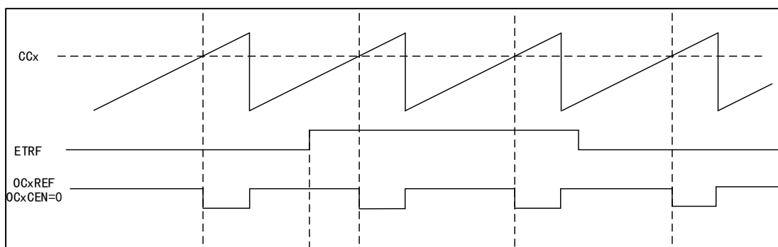
Figure 43 OCxREF Timing Diagram
