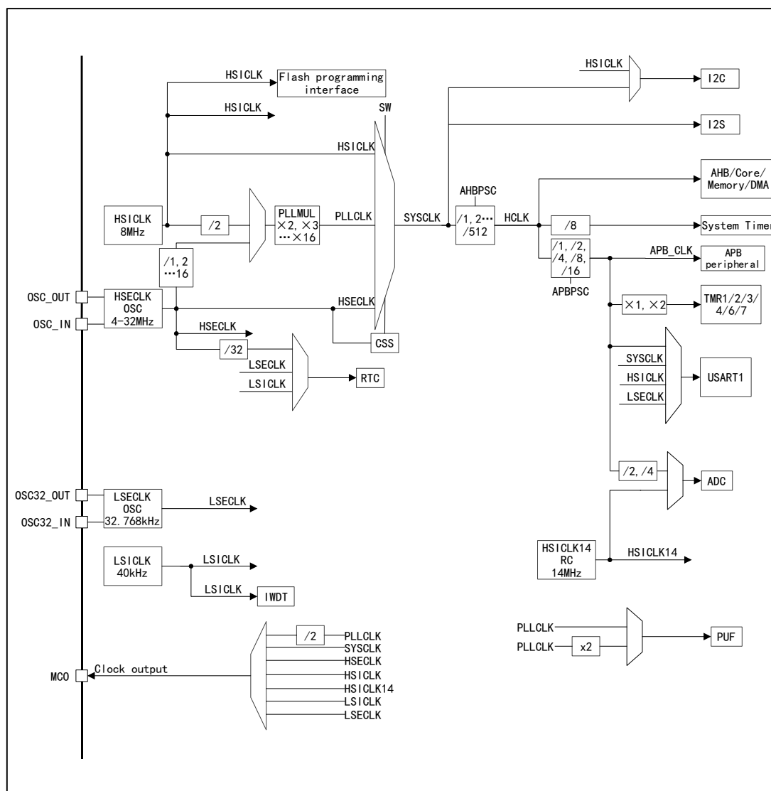
Figure 7 APM32F035x8T7 Clock Tree
