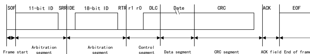
Figure 70 Extended Data Frame
