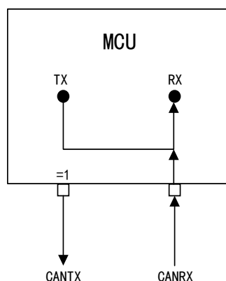
Figure 71 CAN Works in Mute Mode
