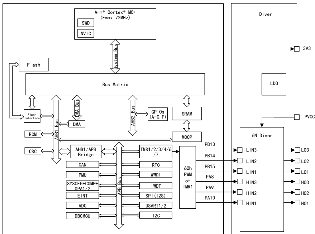
Figure 2 APM32M3514x8 System Architecture Block Diagram
